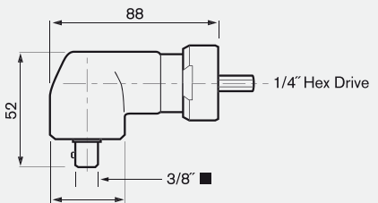
0 607 451 618 Dimensions in mm
