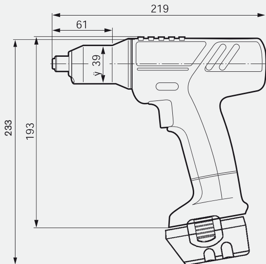
All EXACT, BT-EXACT and SEC-EXACT 9.6 volt models Dimensions in mm
