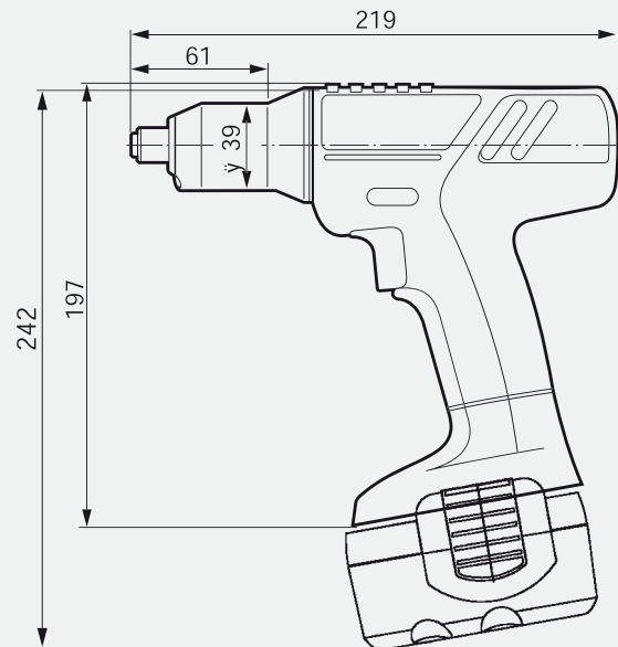
All standard and BT-EXACT 12 volt models Dimensions in mm
