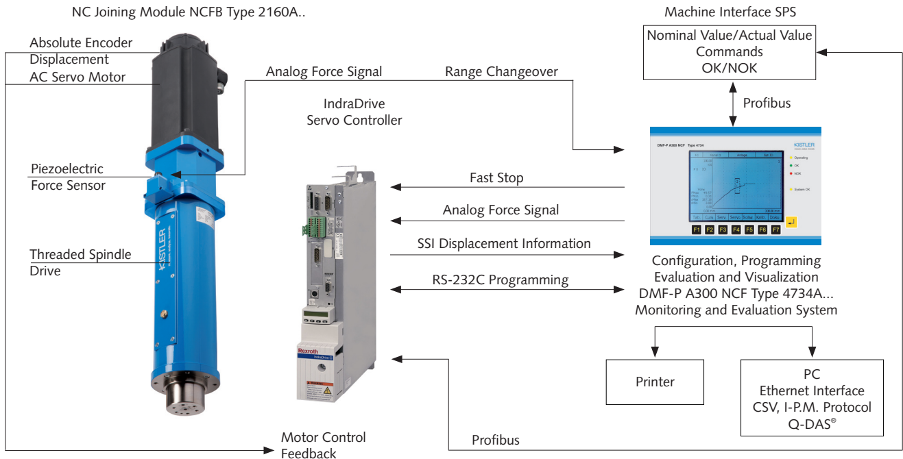
Fig. 3: Functional principle of NC joining system with NC joining module NCFB Type 2160A... and DMF-P A300 NCF Type 4734A...
