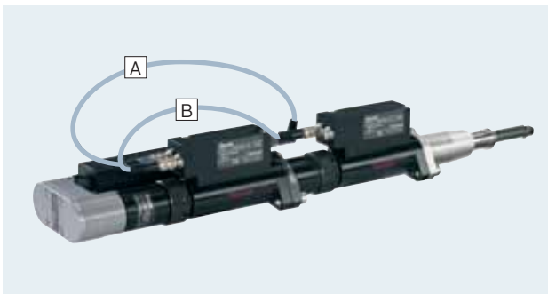
Tightening spindle with transverse gearbox and redundant measurement transducer
